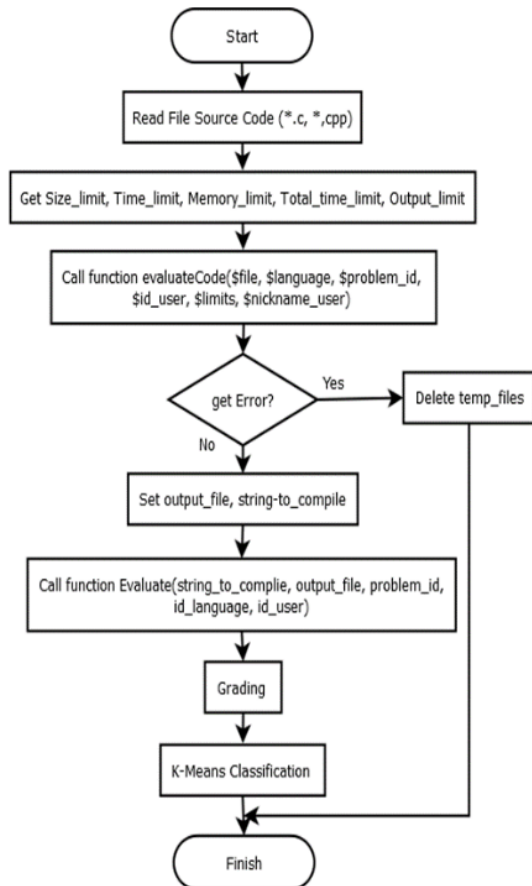
Fig. 1. Flowchart Automatic Assessment
